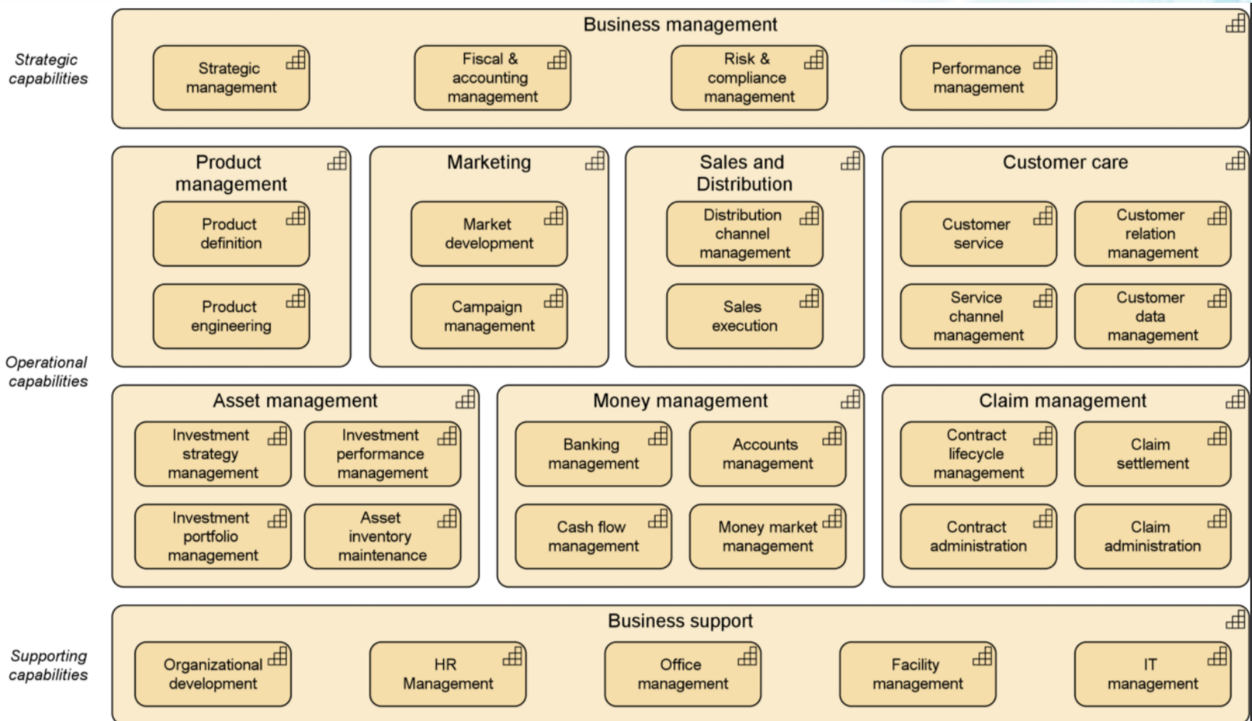
Figure 1. Capability map.
